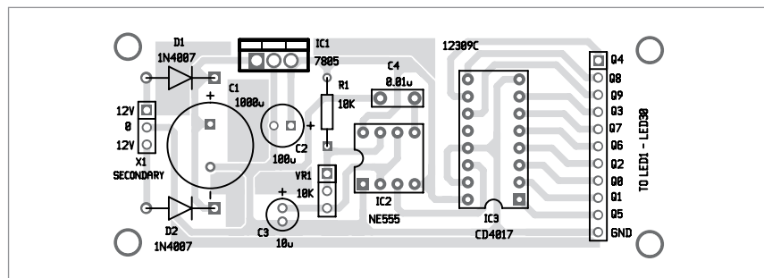
Fig. 4: Components layout of the PCB
